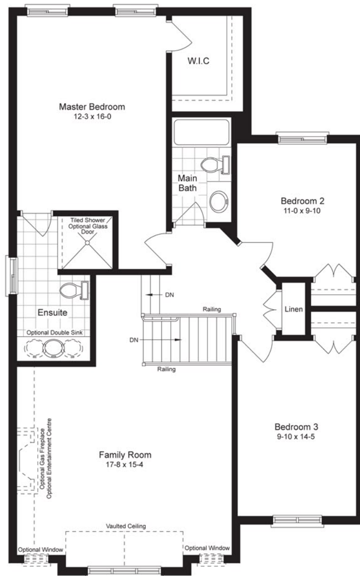
Elevation A Second Floor Plan 3 Bedroom with Upper Family Room
