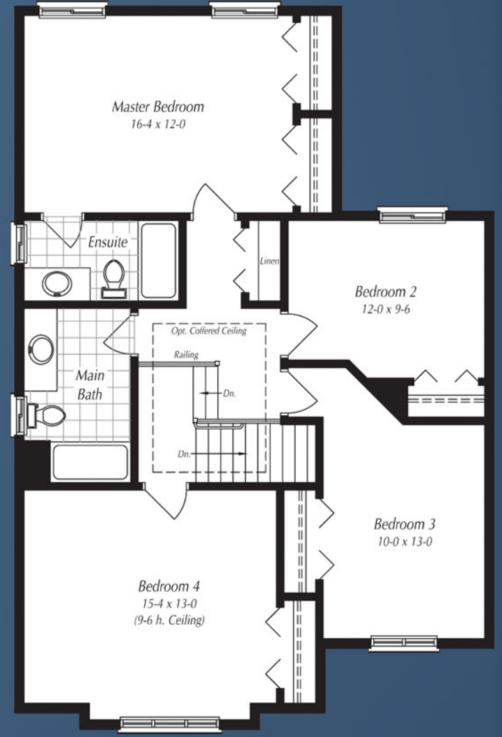
SECOND FLOOR 4 BEDROOM OPTION ELEVATION A
