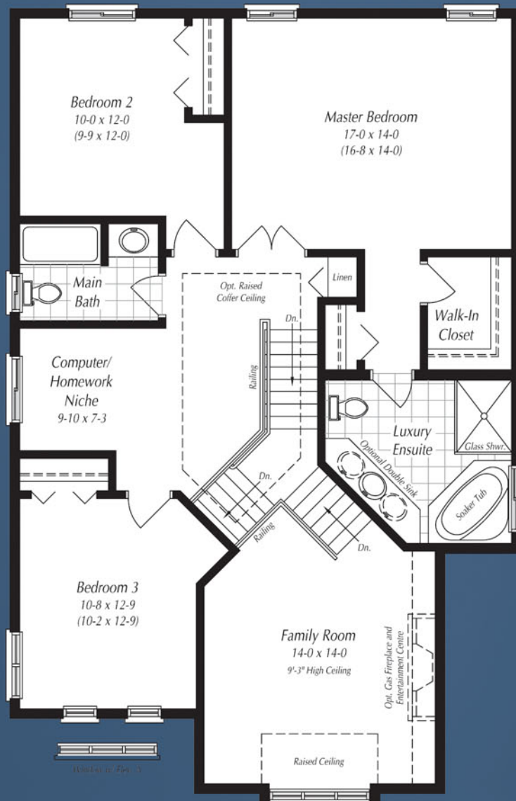
SECOND FLOOR ELEVATION B
