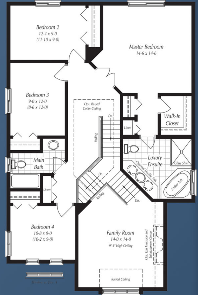
SECOND FLOOR 4 BEDROOM OPTION ELEVATION B
